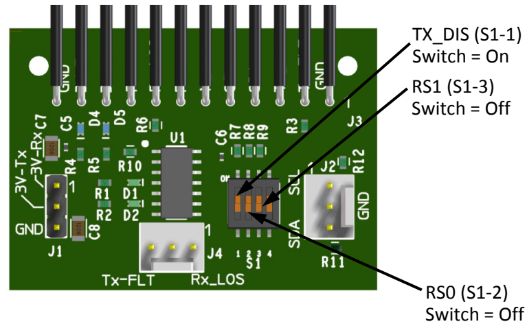
Figure 7. SFP28-TPA-MCB-R Switch Module
