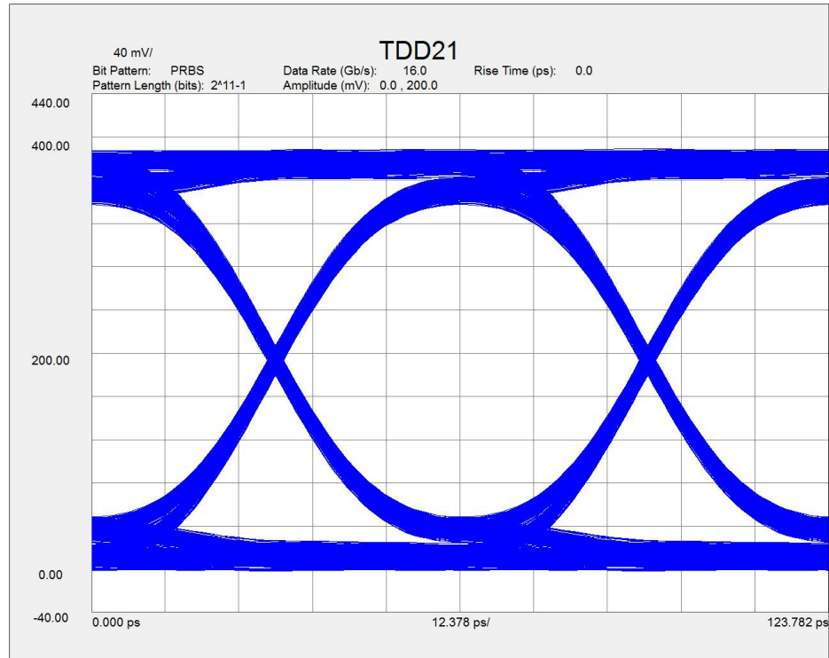
Figure 11. Typical mated pair 16 Gb/s eye diagram.
