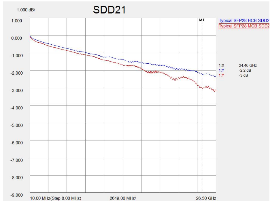
Figure 16. Balanced insertion loss of HCB (blue) without connector, MCB (red) without connector.
