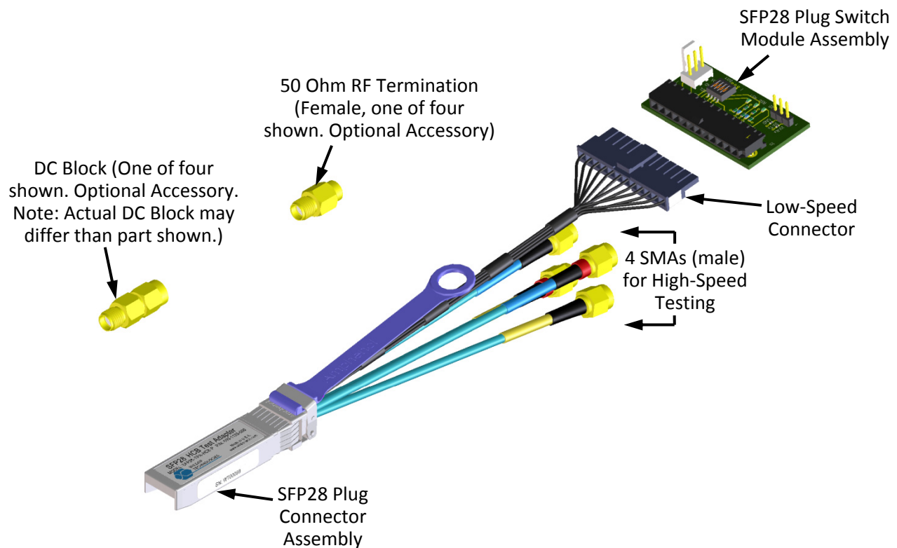
Figure 1. The SFP28 HCB Test Adapter tests to the requirements of the Host Compliance Board (Plug)
