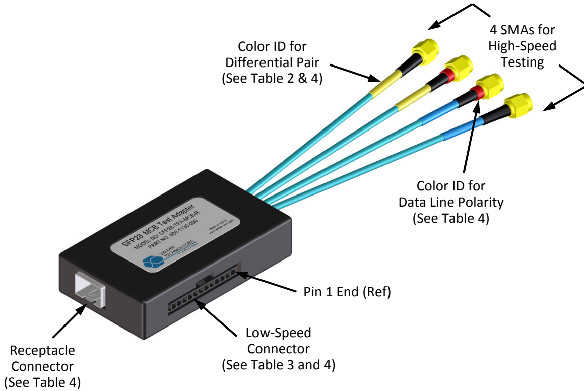
Figure 6. Cable Connectors (SFP28-TPA-MCB-R shown)
