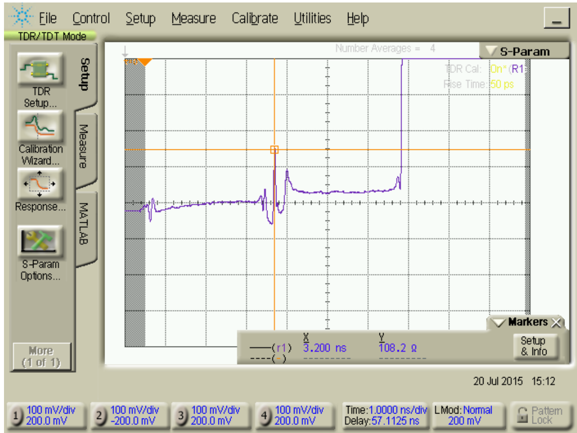
Figure 18. Typical differential TDR of SFP28-TPA-HCB-P connected to SFP28-TPA-MCB-R at 34ps Rise Time (20-80%) (Measured at 50ps 10-90%).
