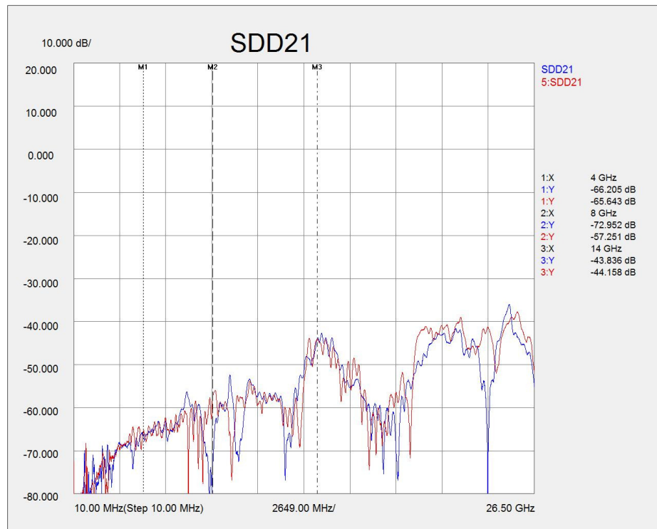
Figure 22. Typical Differential FEXT, with mated connectors, adjacent differential pairs, both transmit and receive terminated at both ends.
