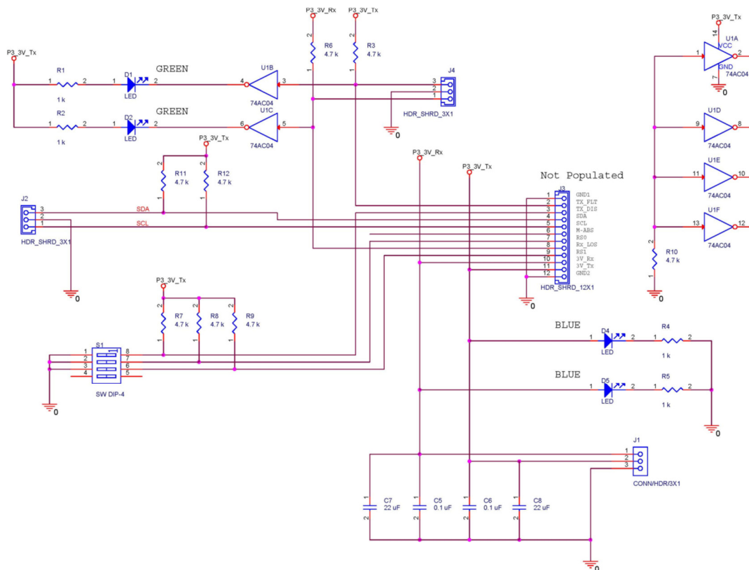
Figure 8. SFP28-TPA-MCB-R Switch Module Schematic
