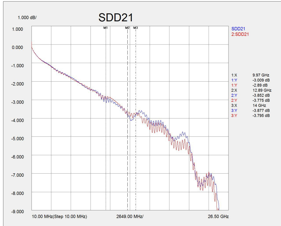
Figure 15. Typical mated pair balanced insertion loss.
