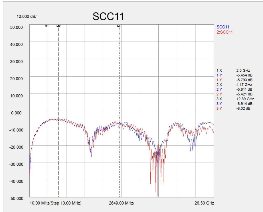
Figure 19. Typical mated pair common mode return loss.
