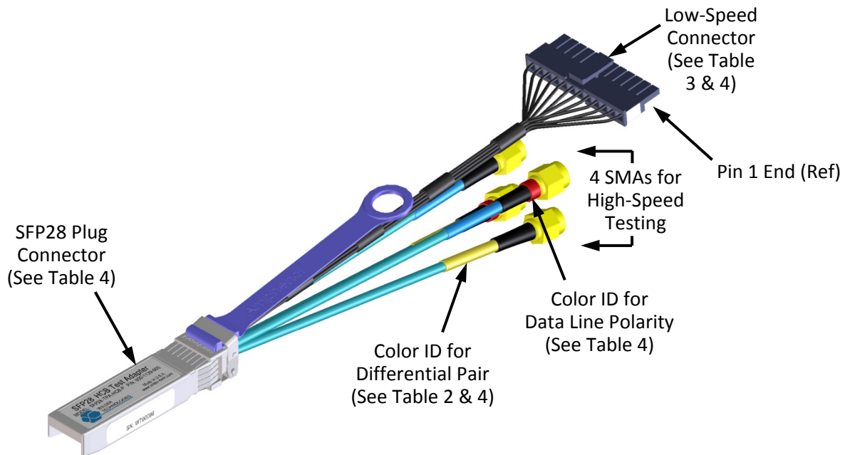
Figure 3. Cable Connectors (SFP28-TPA-HCB-P shown)
