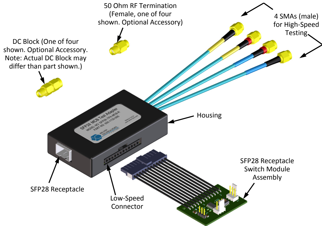
Figure 2. The SFP28 MCB Test Adapter tests to the requirements of the Module Compliance Board (Receptacle)
