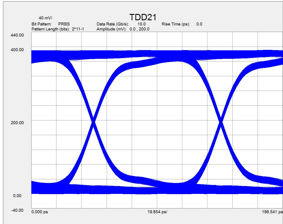
Figure 9. Typical mated pair 10 Gb/s eye diagram.
