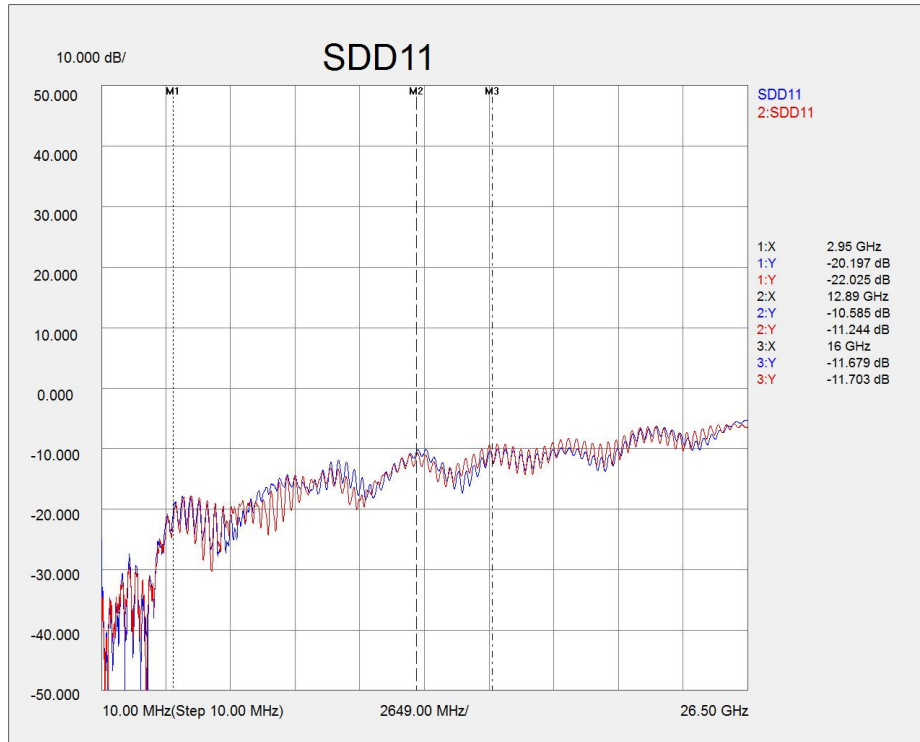
Figure 17. Typical mated pair balanced return loss.
