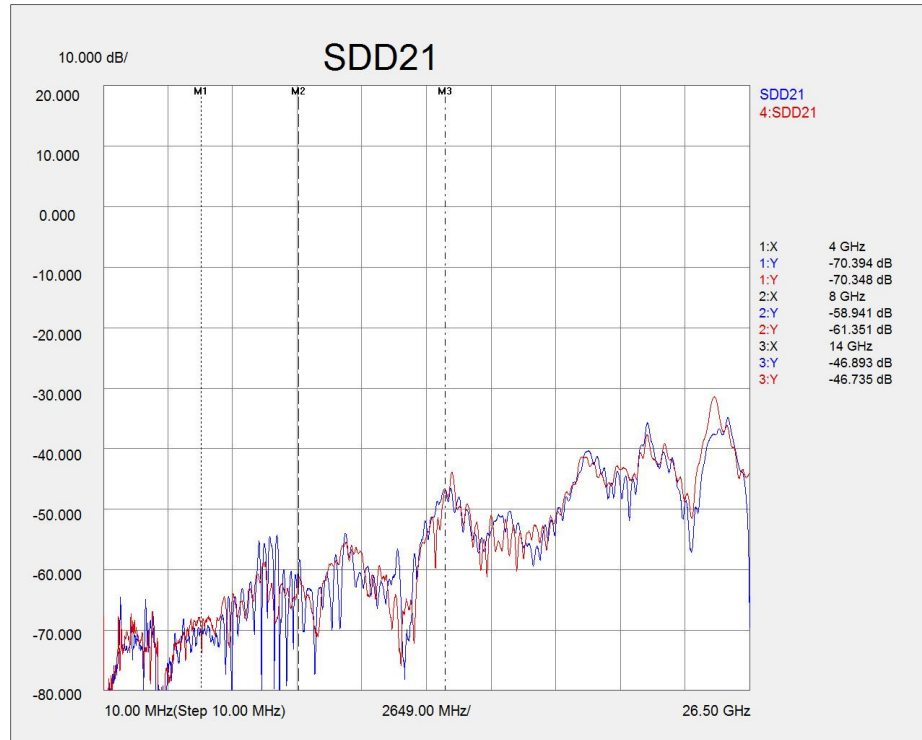
Figure 21. Typical Differential NEXT, with mated connectors, adjacent differential pairs, both transmit and receive terminated at both ends.
