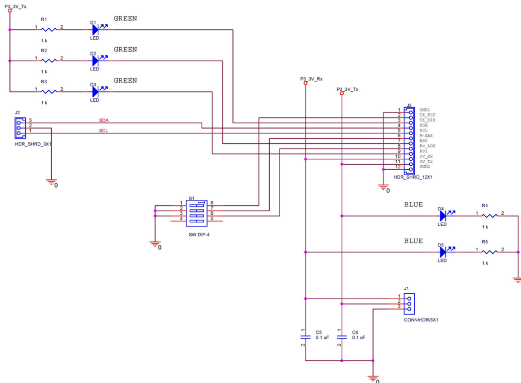
Figure 5. SFP28-TPA-HCB-P Switch Module Schematic
