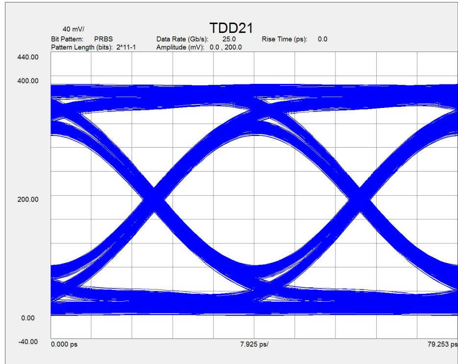
Figure 13. Typical mated pair 25 Gb/s eye diagram.
