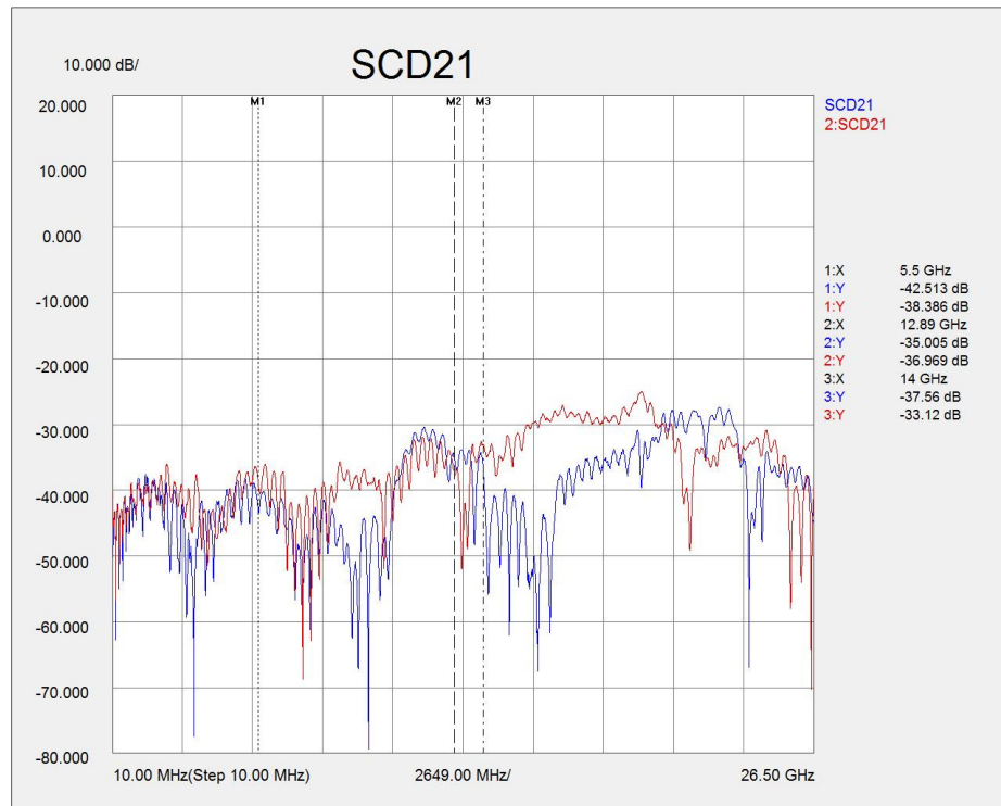
Figure 20. Typical mated pair differential to common mode conversion.
