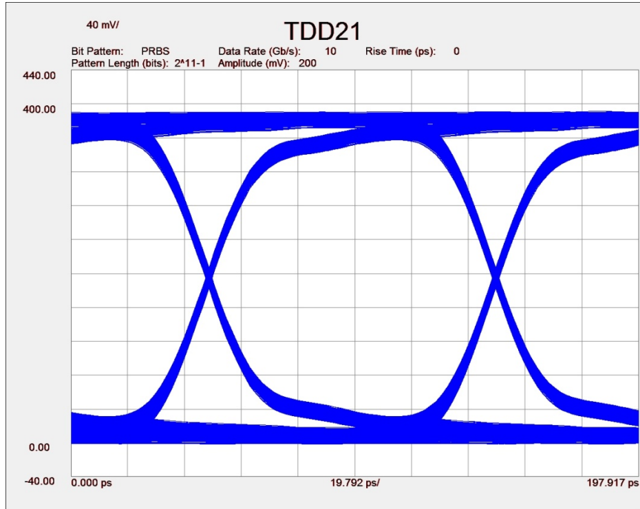
Figure 9. Typical mated pair 10 Gb/s eye diagram.
