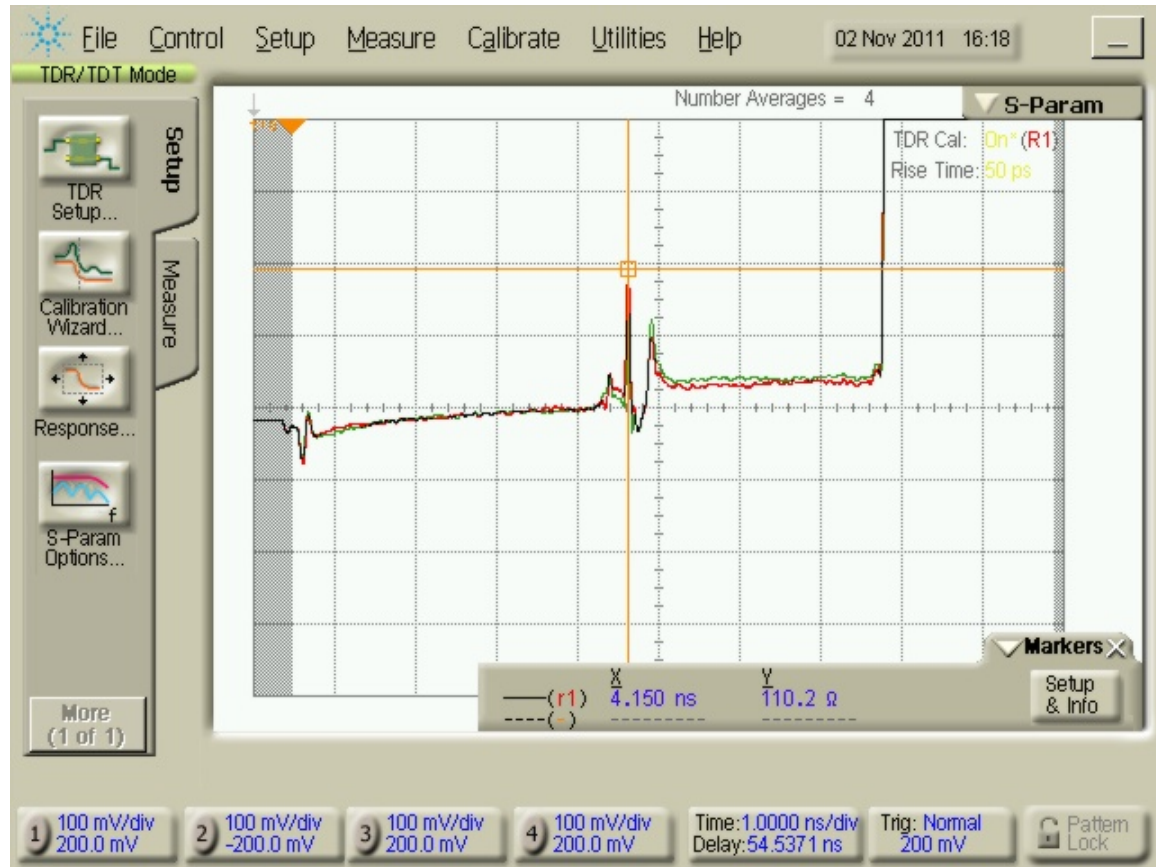
Figure 15. Typical differential TDR of SFP+-TPA-HCB-P connected to SFP+-TPA-MCB-R at 34ps Rise Time (20-80%) (Measured at 50 ps 10-90%).
