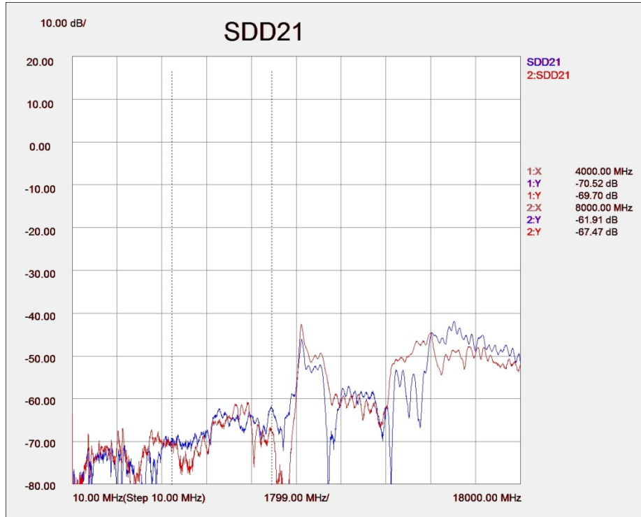
Figure 18. Typical Differential NEXT, with mated connectors, adjacent differential pairs, both transmit and receive terminated at both ends.
