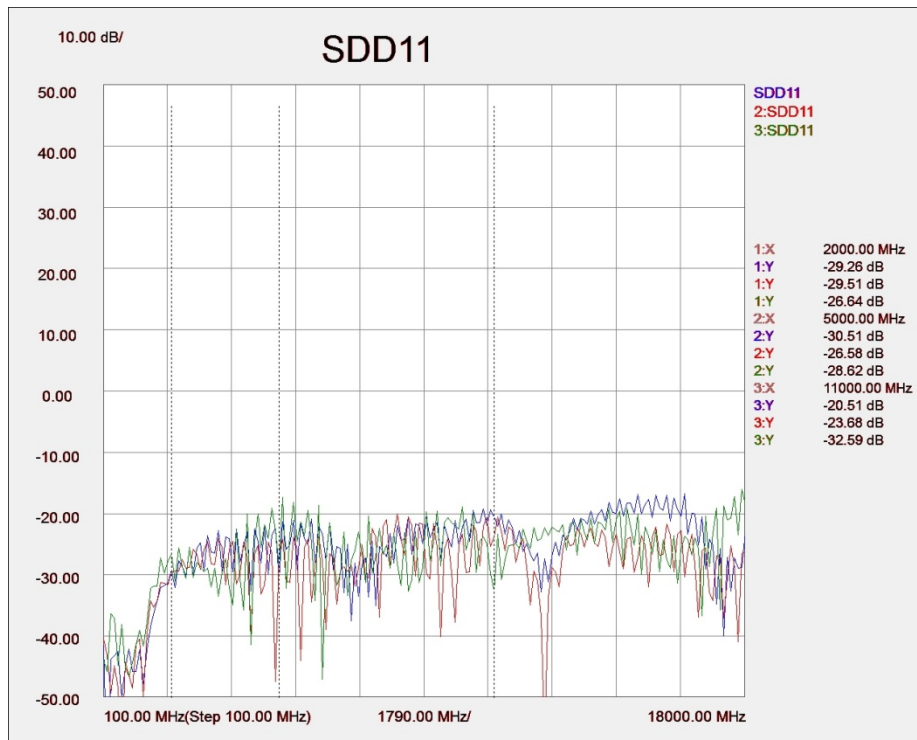
Figure 14. Available S4Ps showing balanced return loss of HCB without connector, MCB without connector, and HCB through MCB without connectors.
