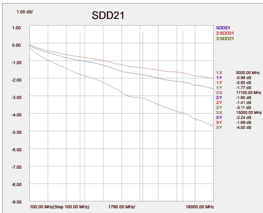
Figure 12. Available S4Ps showing balanced insertion loss of HCB without connector, MCB without connector, and HCB Through MCB without connectors.
