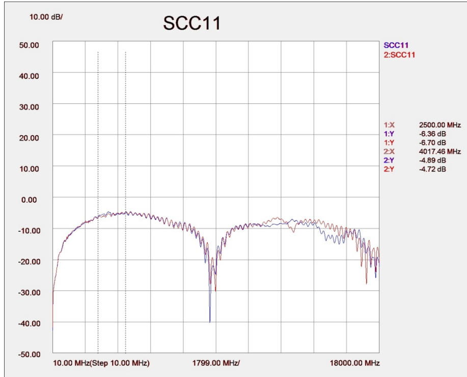
Figure 16. Typical mated pair common mode return loss.
