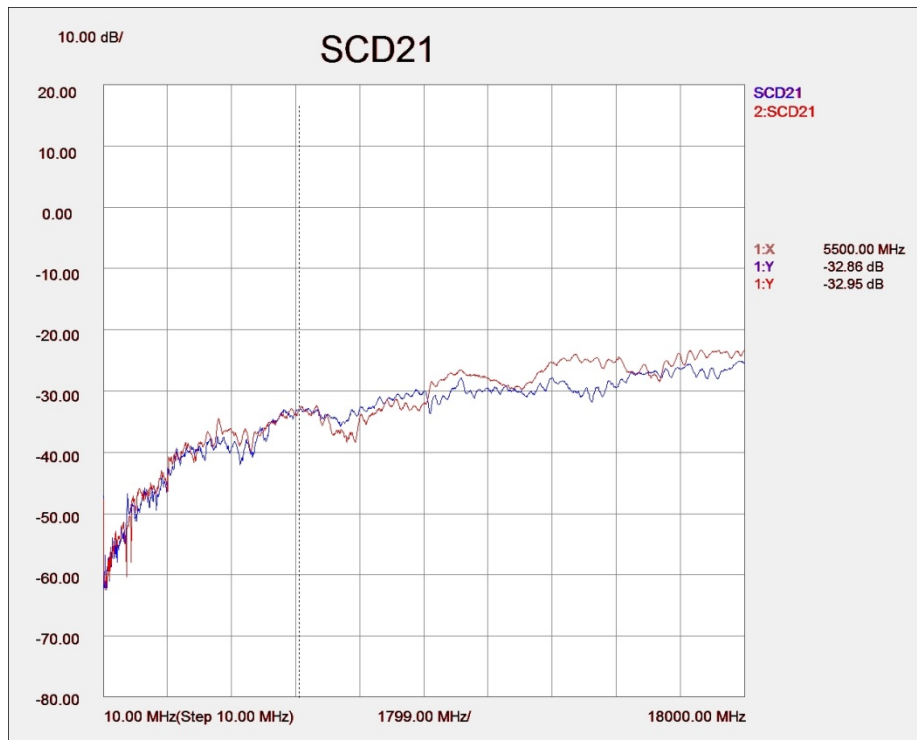
Figure 17. Typical mated pair differential to common mode conversion.
