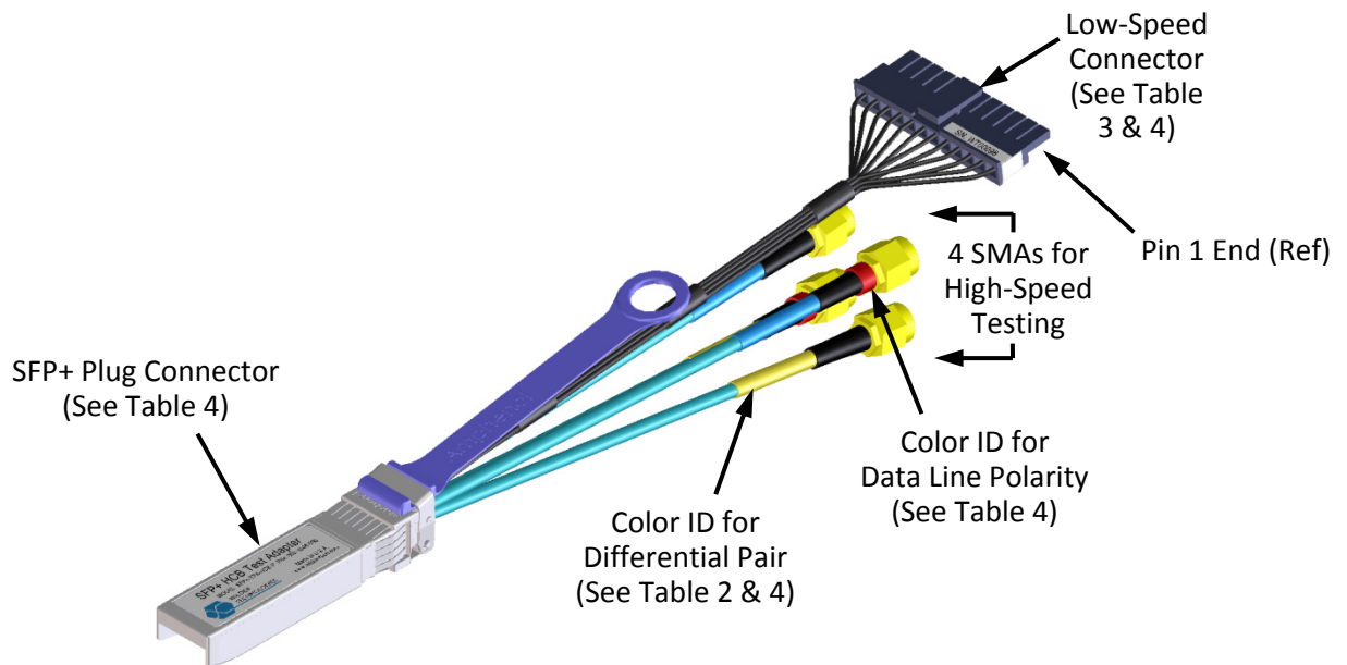
Figure 3. Cable Connectors (SFP+-TPA-HCB-P shown)
