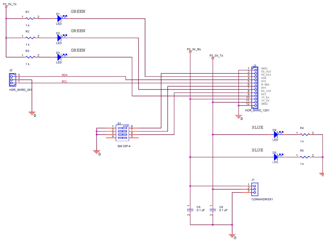
Figure 5. SFP+-TPA-HCB-P Switch Module Schematic
