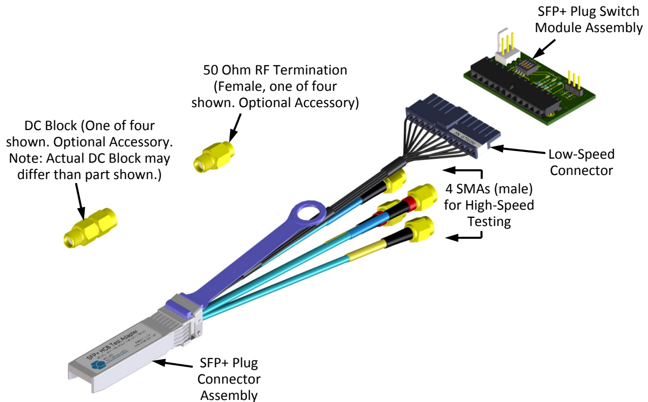
Figure 1. The SFP+ HCB Test Adapter tests to the requirements of the Host Compliance Board (Plug) (Note: Coaxial cables shown are illustrated shorter than those used in the test adapter.)
