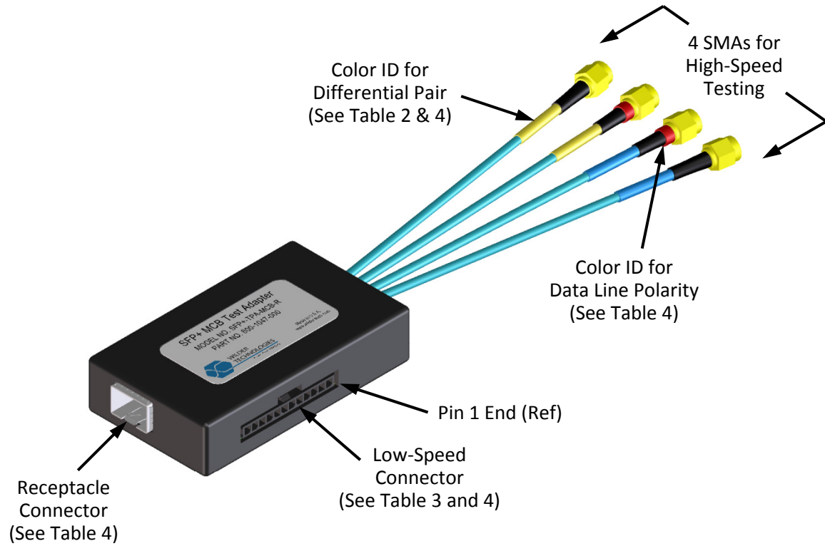
Figure 6. Cable Connectors (SFP+-TPA-MCB-R shown)
