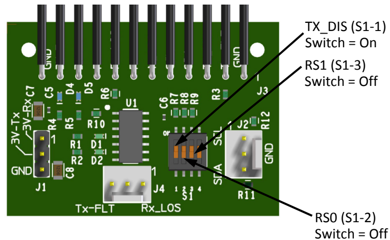
Figure 7. SFP+-TPA-MCB-R Switch Module
