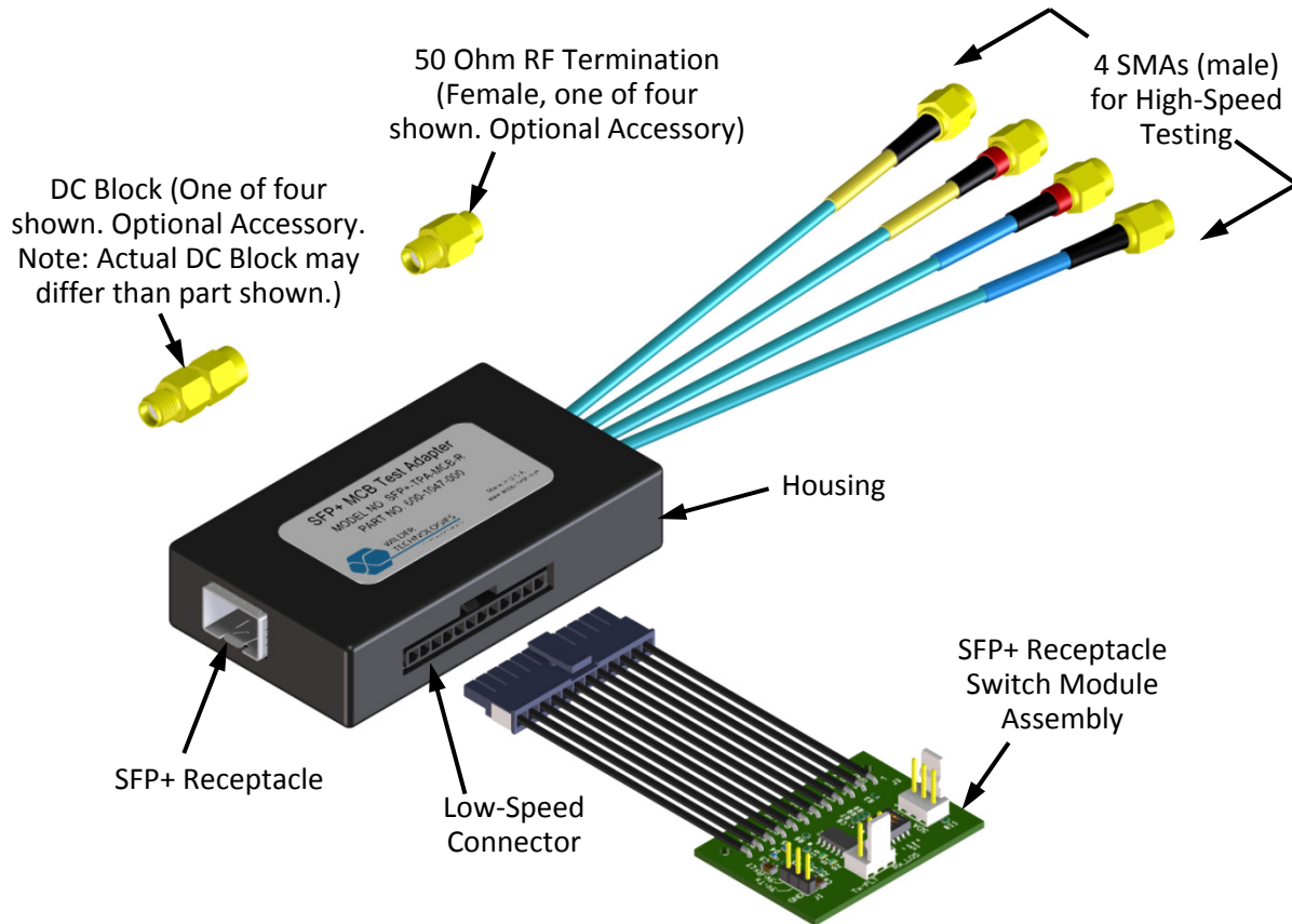
Figure 2. The SFP+ MCB Test Adapter tests to the requirements of the Module Compliance Board (Receptacle)
