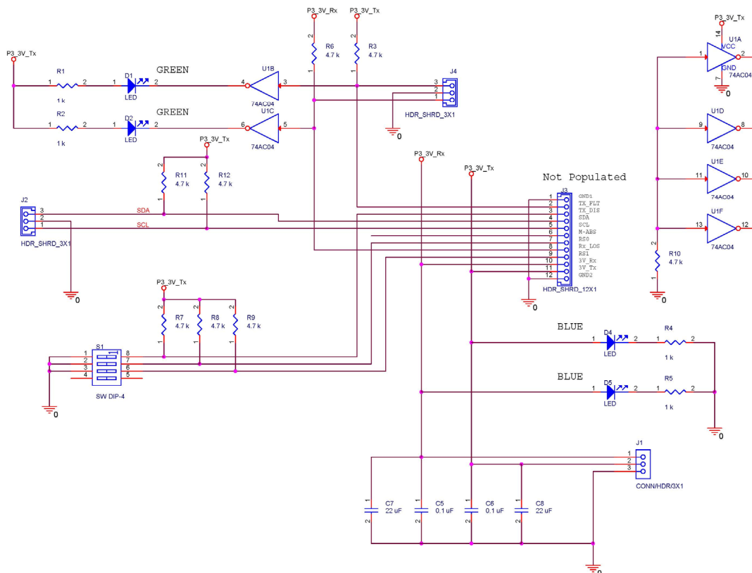
Figure 7. SFP+-TPA-MCB-R Switch Module
