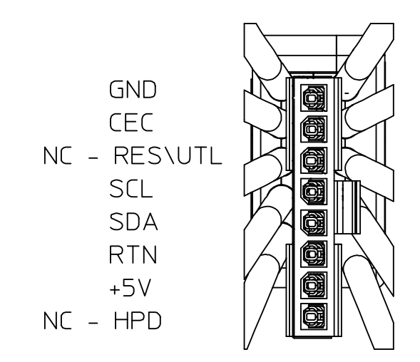
(LOW SPEED CABLE INTERFACE) DETAIL B SCALE 2:1
