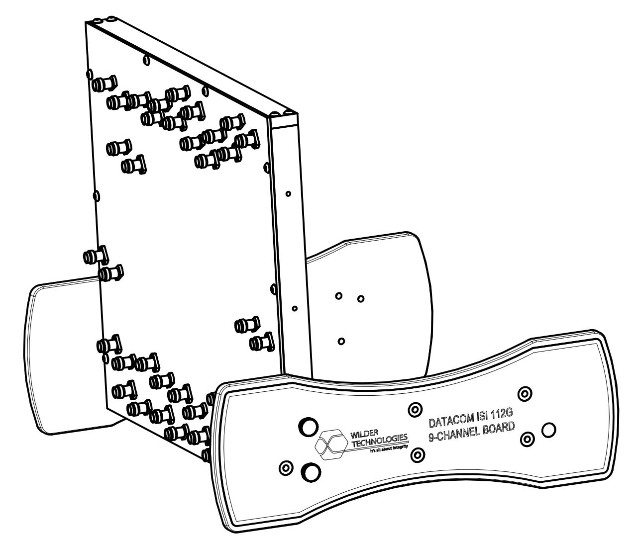
VERTICAL CONFIGURATION SCALE 1:2
