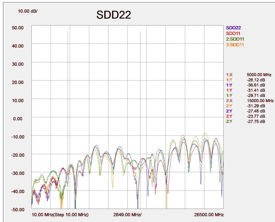
Figure 9. Typical mated board only return loss, receptacle, terminations replacing main connectors.
