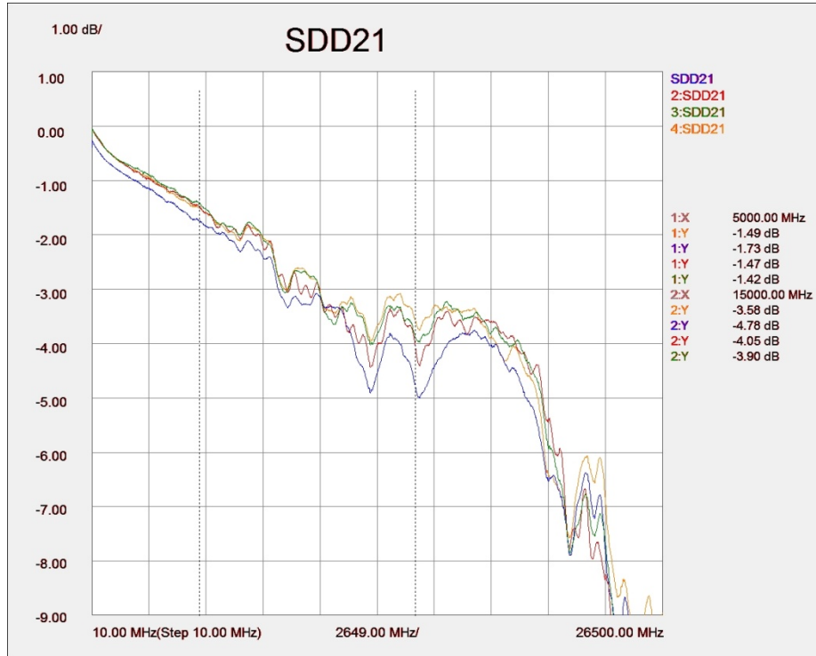
Figure 5. Typical mated pair balanced insertion loss, without calibration.
