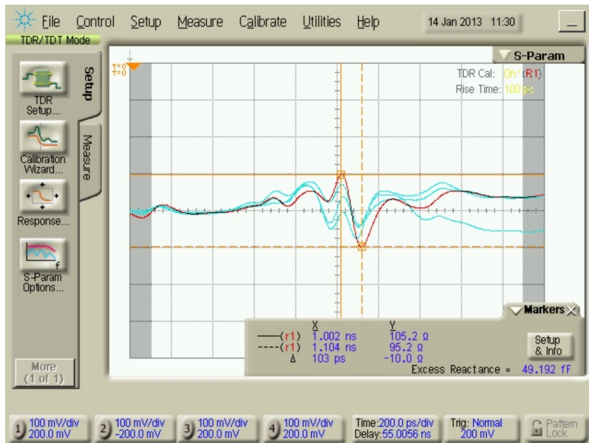
Figure 10. Typical Differential TDR of TPA-ER connected to TPA-P at 100 ps Rise Time. Note- RX0 has 1k ohm sense lines on the plug TPA that impacts the resulting impedance.
