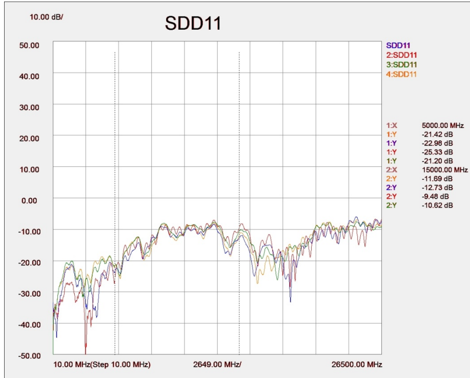
Figure 7. Typical mated pair balanced return loss, without calibration.
