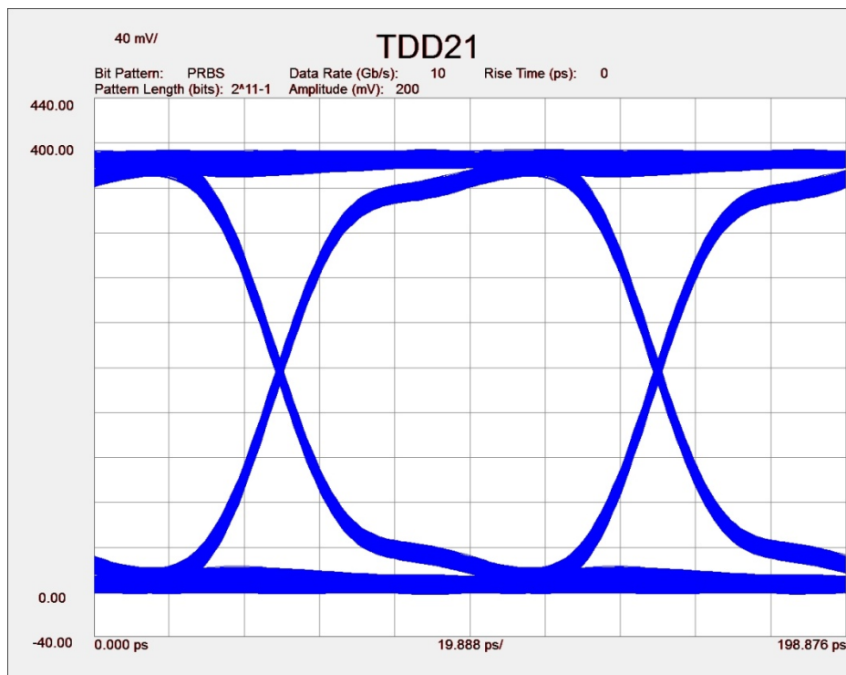
Figure 3. Typical mated pair 10 Gb/s eye diagram, with calibration (top) and without calibration (bottom).
