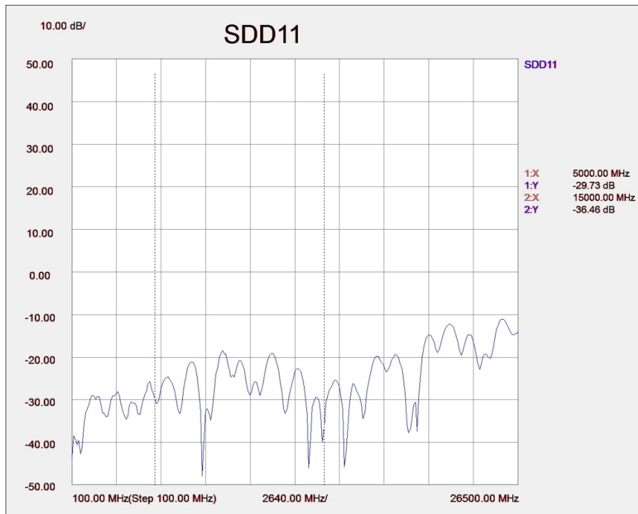
Figure 8. Available S4P showing balanced return loss of ER receptacle from connector traces to SMAs.
