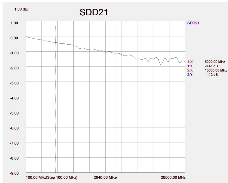
Figure 6. Available S4P showing balanced insertion loss of ER receptacle from connector traces to SMAs.
