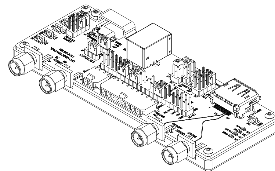
GENERAL VIEW
